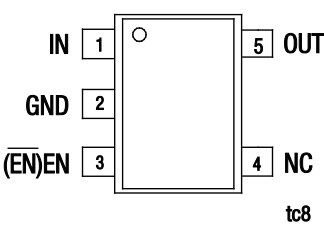
Figure 2. AAT3221 Pinout 5-Pin SOT23-5 (Top View)
