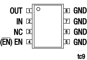
Figure 3. AAT3221 Pinout 8-Pin SC70JW-8 (Top View)
