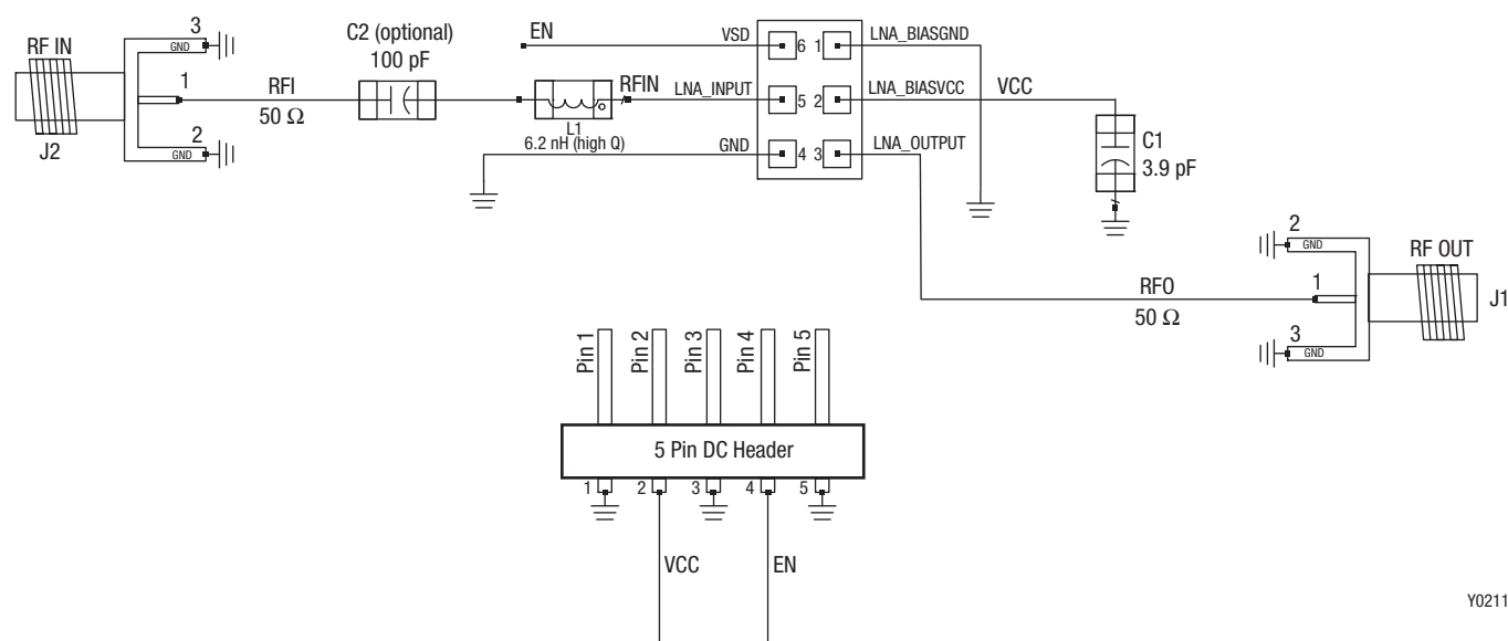
Figure 3. SKY65605-21 Evaluation Board Schematic
