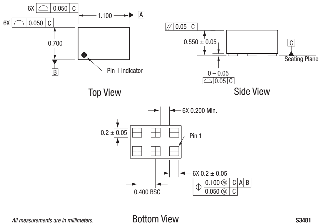
Figure 6. SKY65605-21 Package Dimensions
