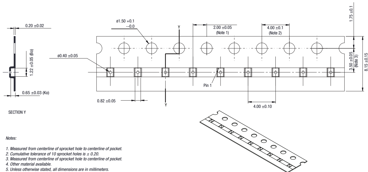
Figure 7. SKY65605-21 Tape and Reel Dimensions
