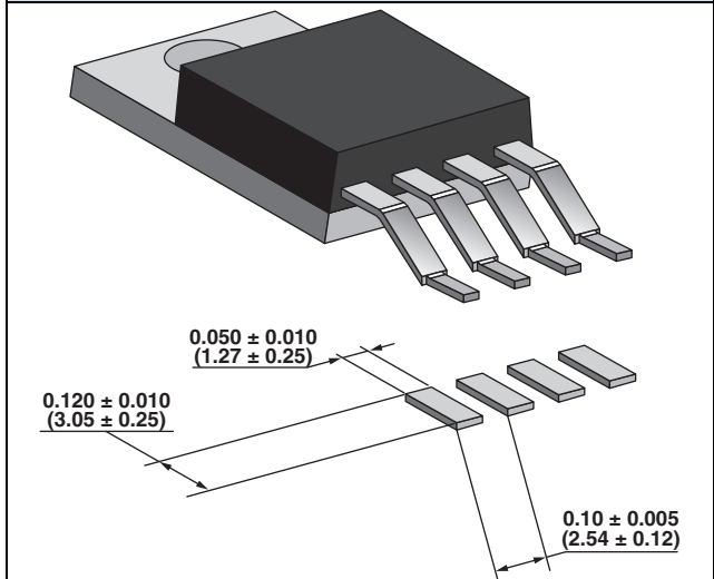
FIGURE 8 - VPR221S LAND PATTERN DIMENSIONS in inches (millimeters)
