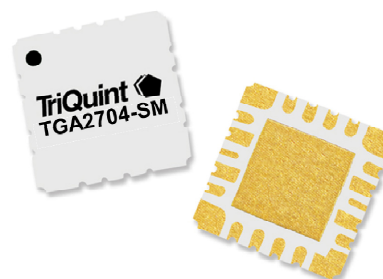
QFN 7x7mm 22L
