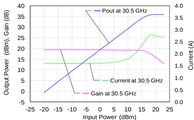
30.5 GHz Power, Gain, and Current vs. Input Power
