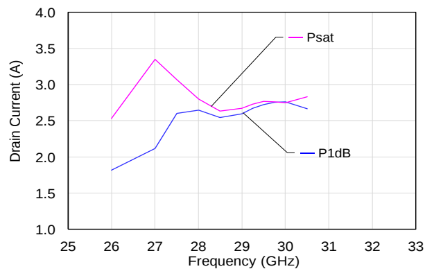
Drain Current vs. Frequency
