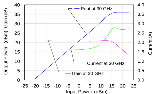
30 GHz Power, Gain, and Current vs. Input Power
