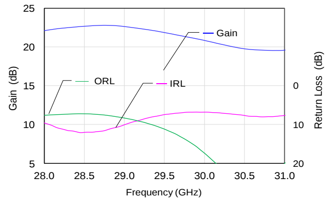
S-Parameters vs. Frequency
