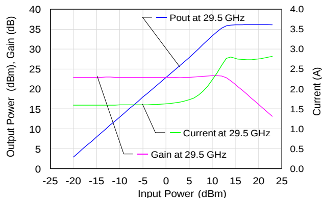
29.5 GHz Power, Gain, and Current vs. Input Power
