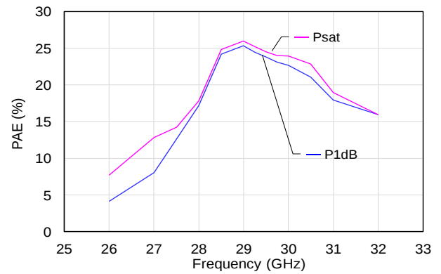
Power Added Efficiency vs. Frequency
