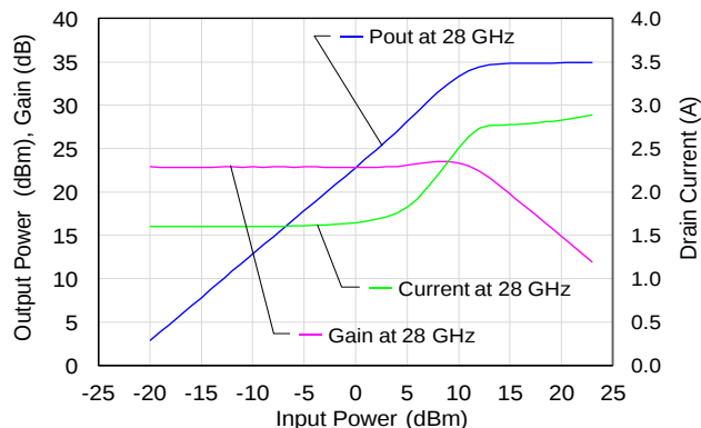
28 GHz Power, Gain, and Current vs. Input Power
