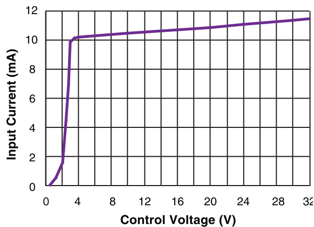
Figure 3c — SH60D relays
