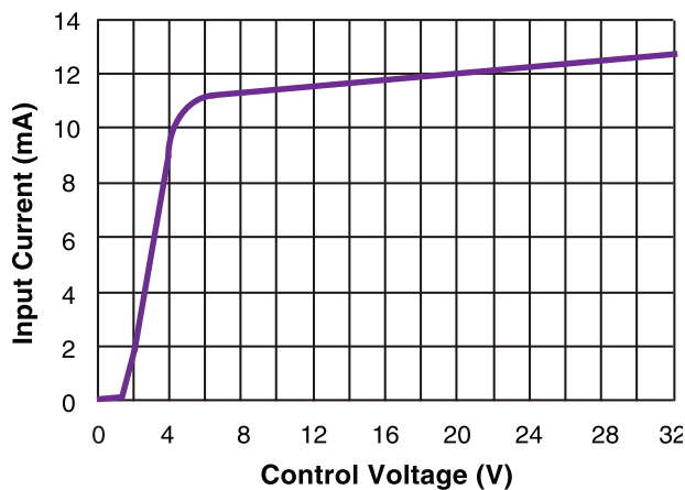
Figure 3a — SH24R/D, SH48R/D relays
