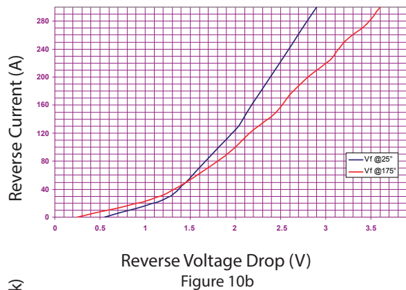
OUTPUT RELAY CHARACTERISTIC CURVES FOR SI170DC25
