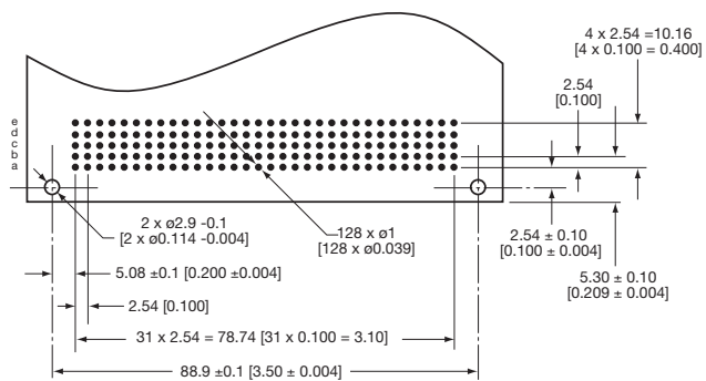
HOLE PATTERN
