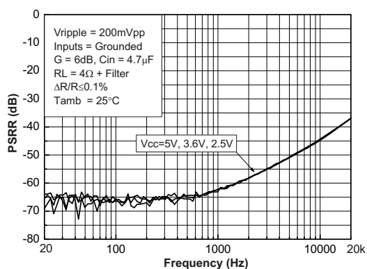
Figure 18. PSRR vs. frequency at R_L = 4\ \Omega + filter
