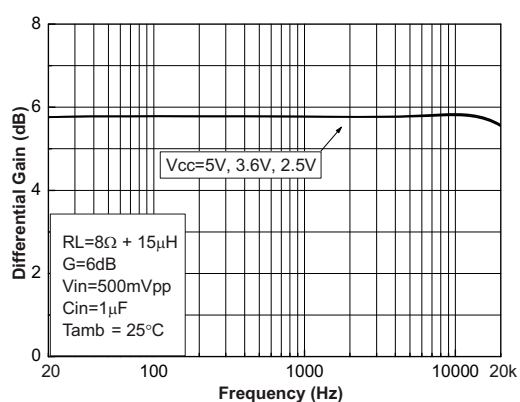
Figure 53. Gain vs. frequency at R_L = 8\ \Omega + 15\ \mu\text{H}
