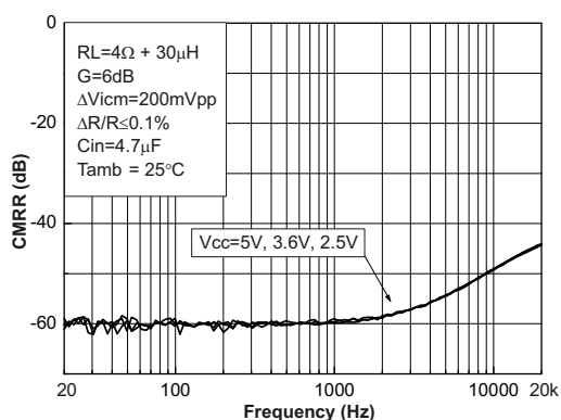
Figure 24. CMRR vs. frequency at R_L = 4\ \Omega + 30\ \mu\text{H}
