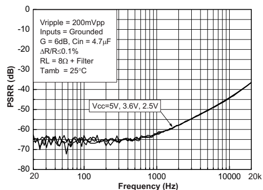
Figure 21. PSRR vs. frequency at R_L = 8\ \Omega + filter
