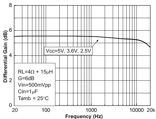
Figure 50. Gain vs. frequency at R_L = 4\ \Omega + 15\ \mu\text{H}
