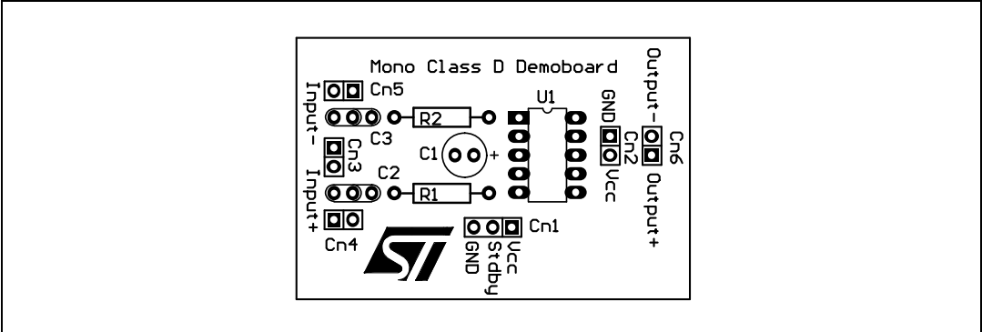
Figure 70. Top view
