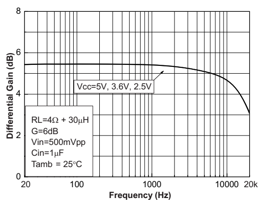
Figure 51. Gain vs. frequency at R_L = 4\ \Omega + 30\ \mu\text{H}
