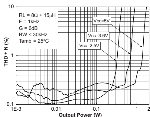
Figure 36. THD+N vs. output power at R_L = 8\ \Omega + 15\ \mu\text{H} , F = 1\ \text{kHz}
