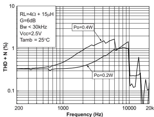
Figure 42. THD+N vs. frequency at R_L = 4\ \Omega + 15\ \mu\text{H} , V_{CC} = 2.5\ \text{V}
