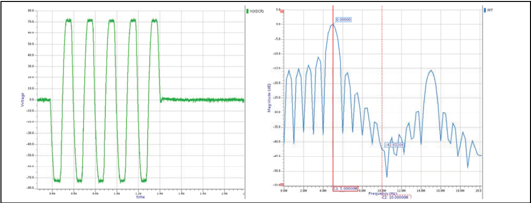
Figure 7. PW and HD2 example (HVP0=80 V, HVM0=-80 V load 300 pF//100 Ω)
