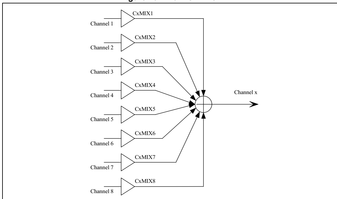
Figure 10. Channel mixer
