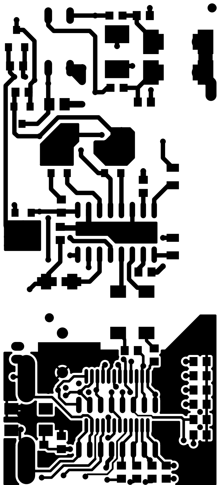
Figure 41. Daughter Card Primary Side
