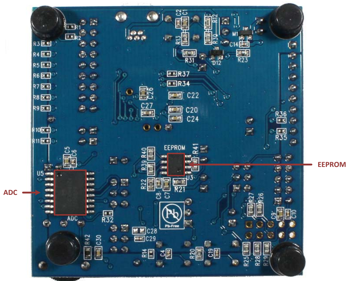
Figure 18. CP2130 Evaluation Board Features (Back)
