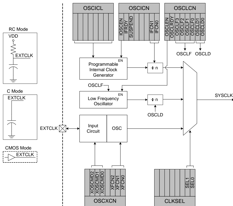
Figure 19.1. Oscillator Options
