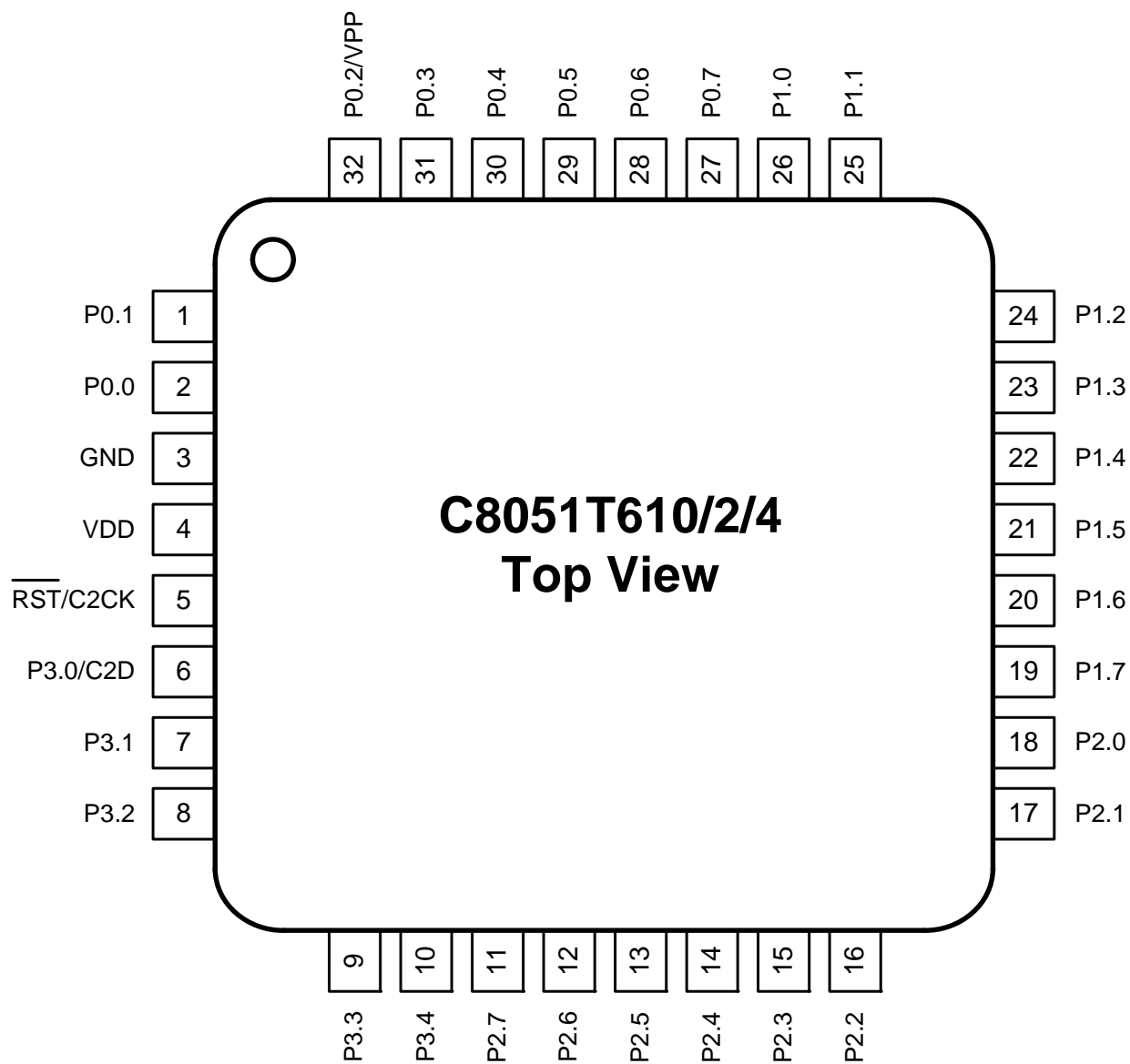
Figure 3.1. LQFP-32 Pinout Diagram (Top View)
