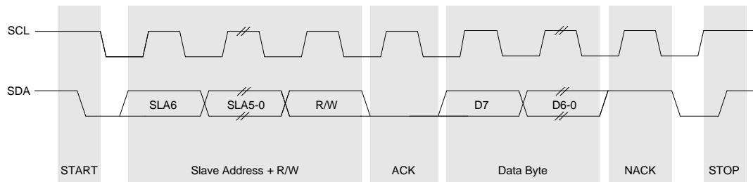
Figure 22.3. SMBus Transaction
