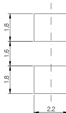
Recommended Solder Pattern
