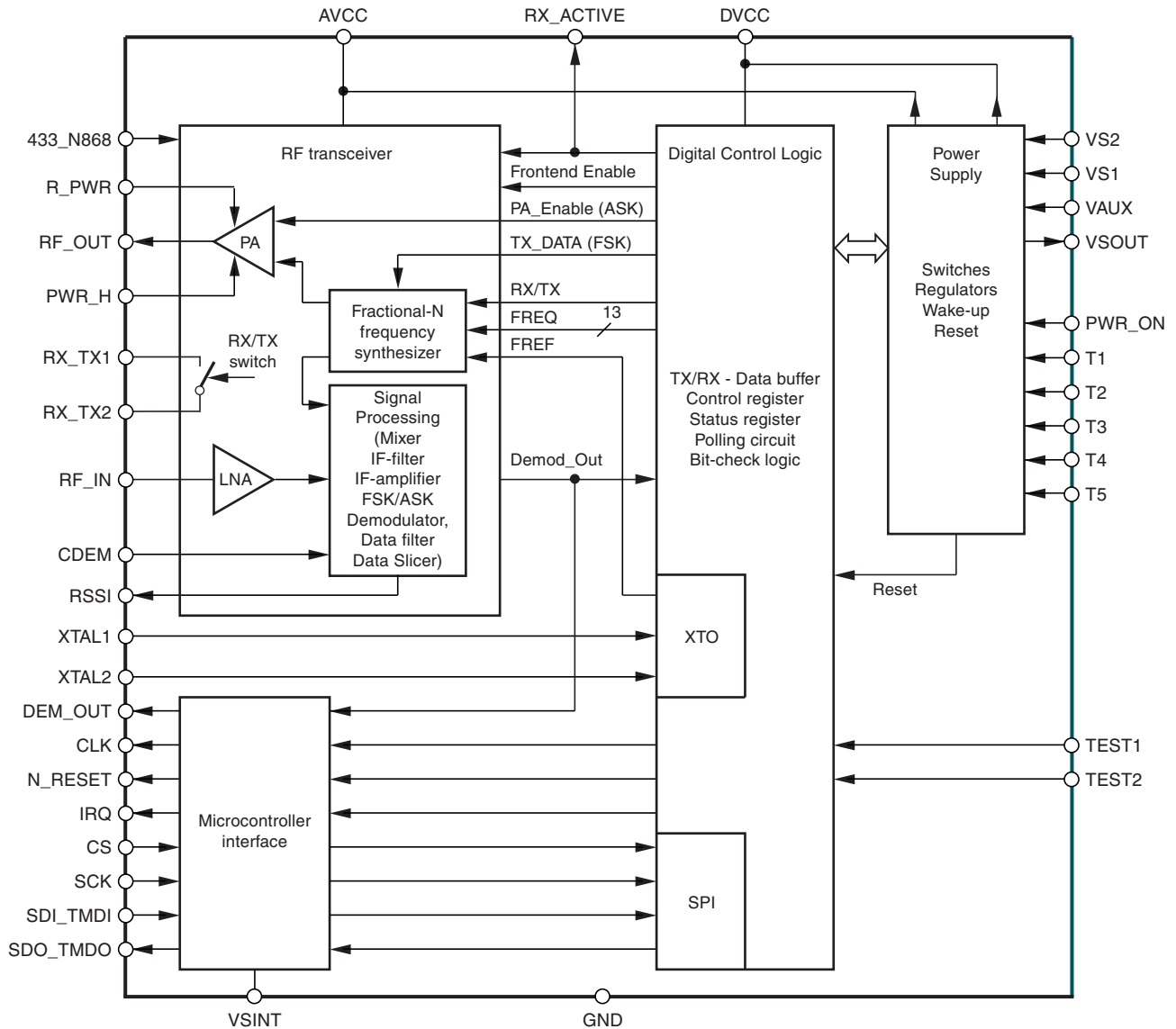
Figure 1-3. Block Diagram
