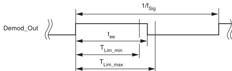
Figure 9-4. Valid Time Window for Bit Check
