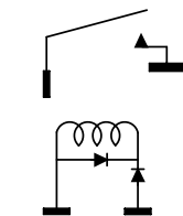
1 FORM A AC OPERATED 1/2 WAVE RECTIFIED (TOP VIEW) Fig. C
