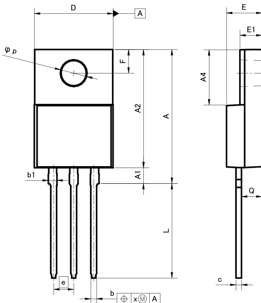
TO-220FM
