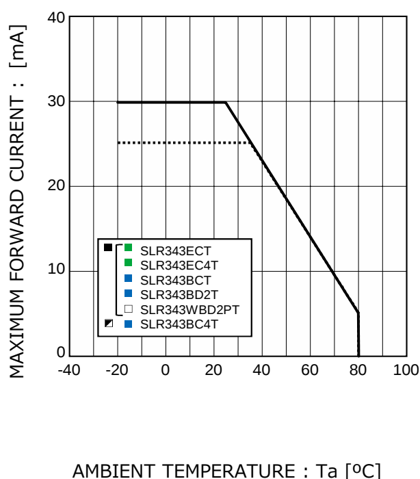
Fig.4 Derating
