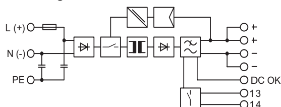
Figure 2 Block diagram
