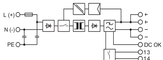
Figure 2 Block diagram
