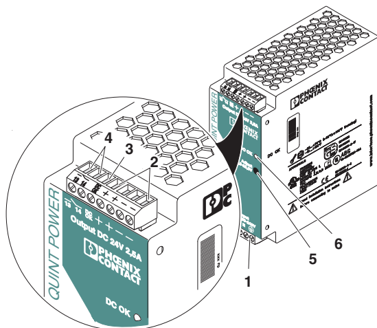
Figure 1 Operating elements
