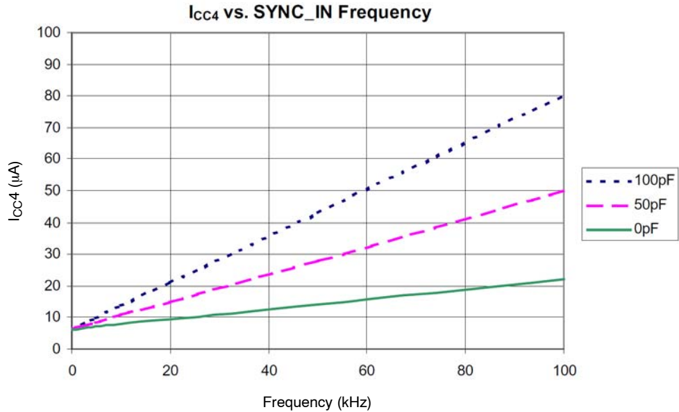
Figure 2. I_{CC4} vs. SYNC_IN Frequency Performance Data
