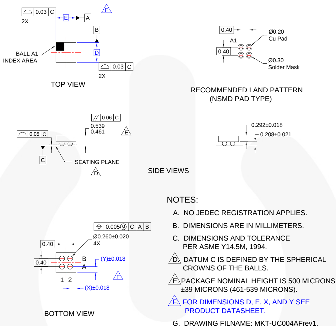
Figure 5. 4-Lead, Wafer-Level Chip Scale 0.76x0.76x0.5mm Wafer-Level Chip-Scale Package (WLCSF)
