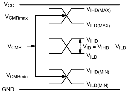
Figure 10. V_{CM} Diagram
