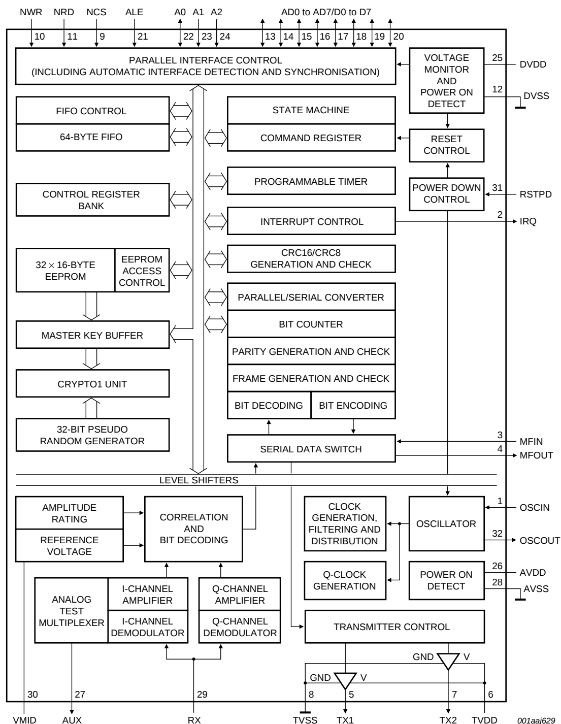
Fig 1. MFRC500 block diagram
