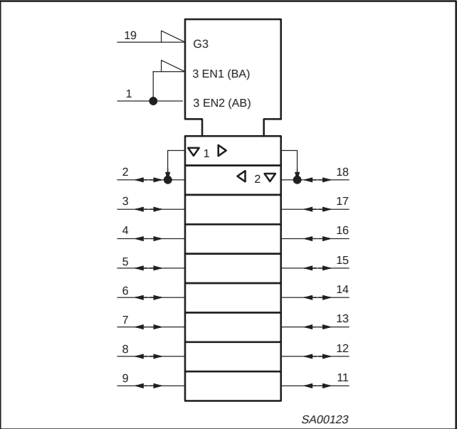
LOGIC SYMBOL (IEEE/IEC)
