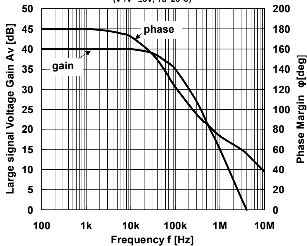
Large signal Voltage Gain vs. Frequency ( V^+/V^-=\pm 5\text{V} , T_a=25^\circ\text{C} )
