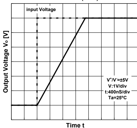
Slew Rate(Rise)
