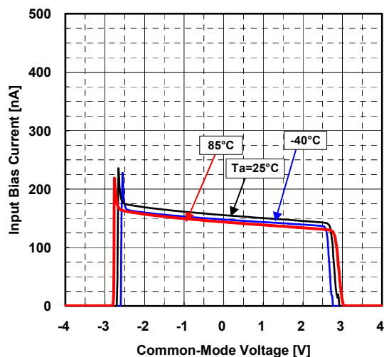
Input Bias Current vs. Input Common-Mode Voltage (Temperature) V^+/V^-\approx\pm 3.5V
