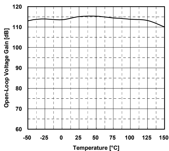
Open-Loop Voltage Gain vs. Temperature R_L=2k\Omega to 0V, V^+/V^-\approx\pm 16V, V_o=-11V to +11V
