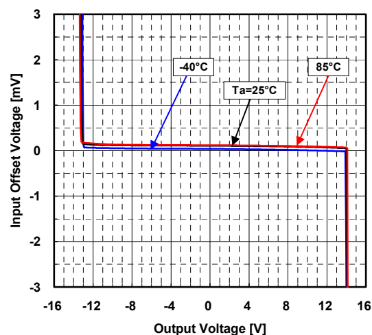
Input Offset Voltage vs. Output Voltage (Temperature) V^+/V^-\approx\pm 15V, R_L=2k\Omega to 0V
