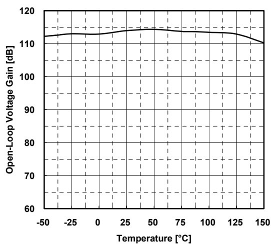
Open-Loop Voltage Gain vs. Temperature R_L=2k\Omega to 0V, V^+/V^-\approx\pm 15V, V_o=-10V to +10V
