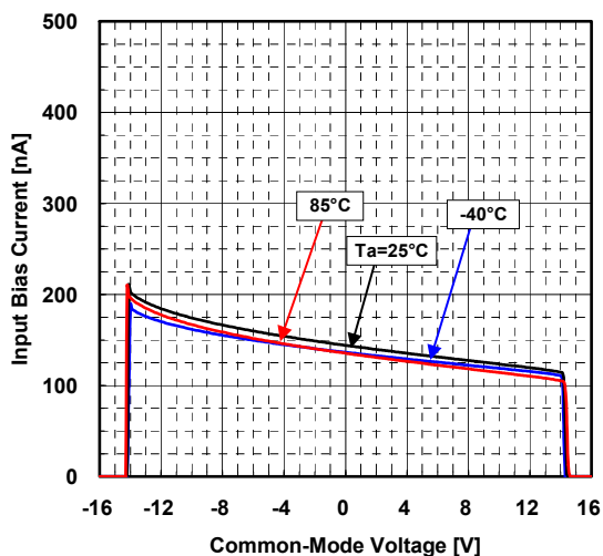
Input Bias Current vs. Input Common-Mode Voltage (Temperature) V^+/V^-\approx\pm 15V
