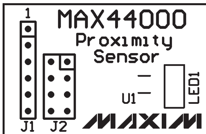
Figure 2. MAX44000PMB11 Peripheral Module Component Placement Guide—Component Side
