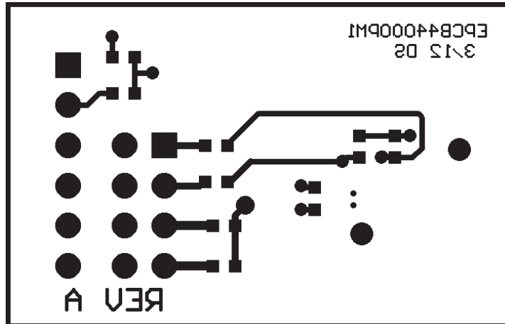
Figure 6. MAX44000PMB11 Peripheral Module PCB Layout—Solder Side
