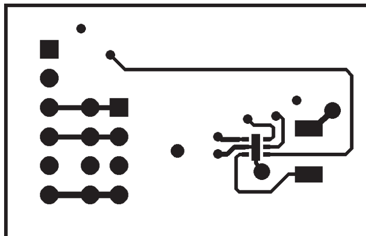
Figure 3. MAX44000PMB11 Peripheral Module PCB Layout—Component Side
