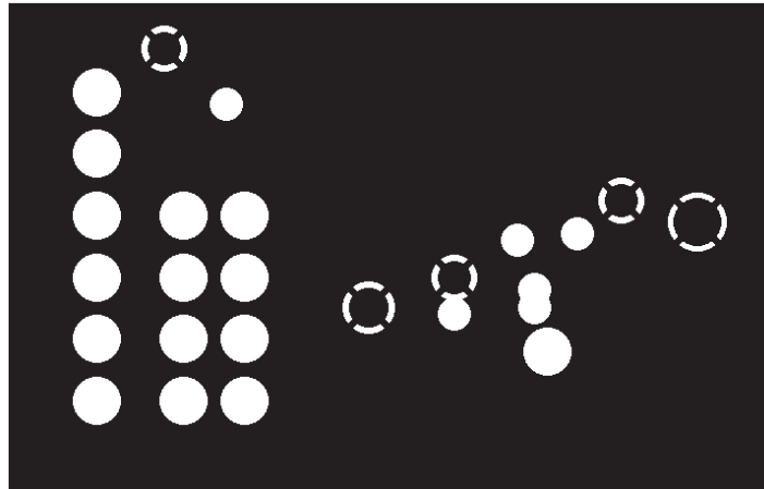
Figure 5. MAX44000PMB11 Peripheral Module PCB Layout—Inner Layer 2 (Power)
