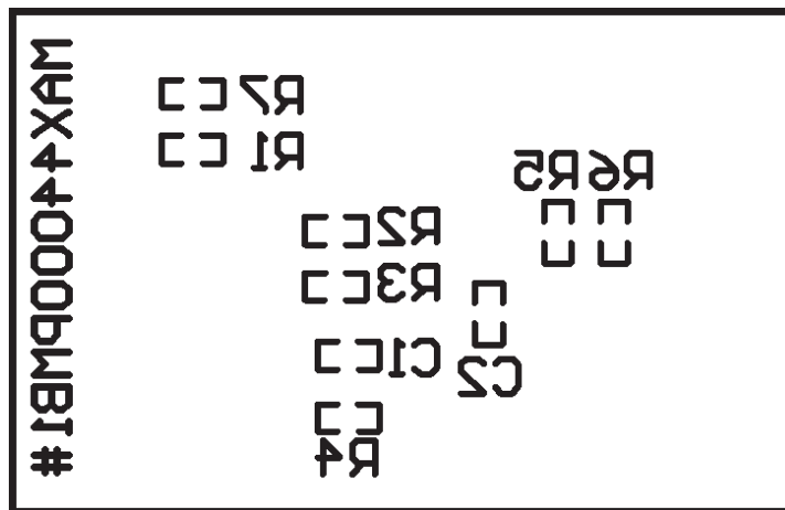
Figure 7. MAX44000PMB11 Peripheral Module Component Placement Guide—Solder Side
