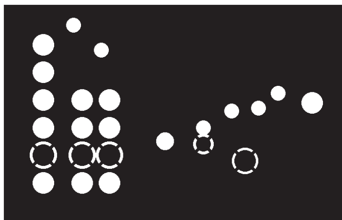
Figure 4. MAX44000PMB11 Peripheral Module PCB Layout—Inner Layer 1 (Ground)
