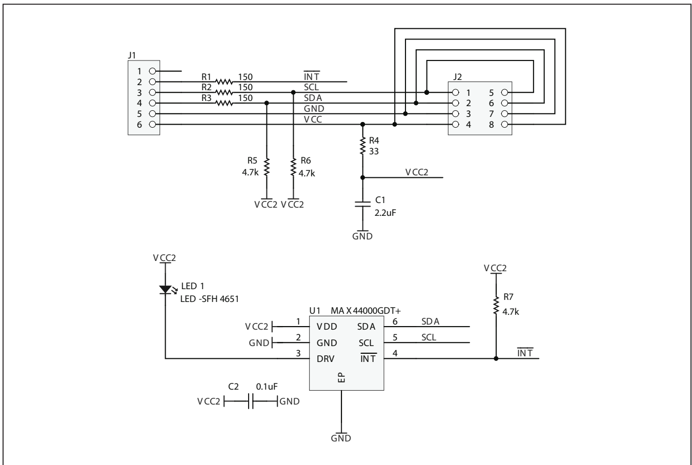
Figure 1. MAX44000PMB1 Peripheral Module Schematic
