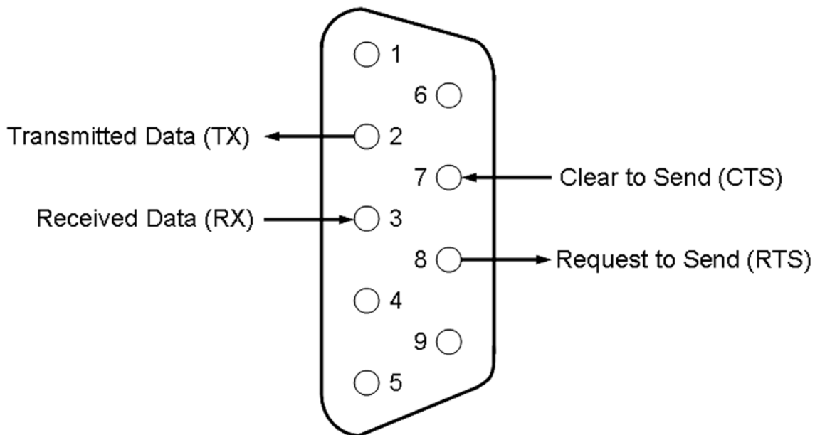
Figure 2. EV Kit J1 Female DB9 Connector Pin Functions
