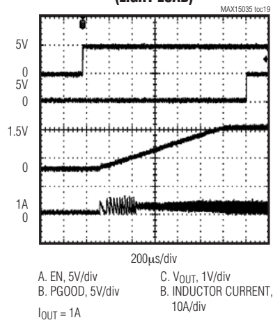
SOFT-START WAVEFORM (LIGHT LOAD)
