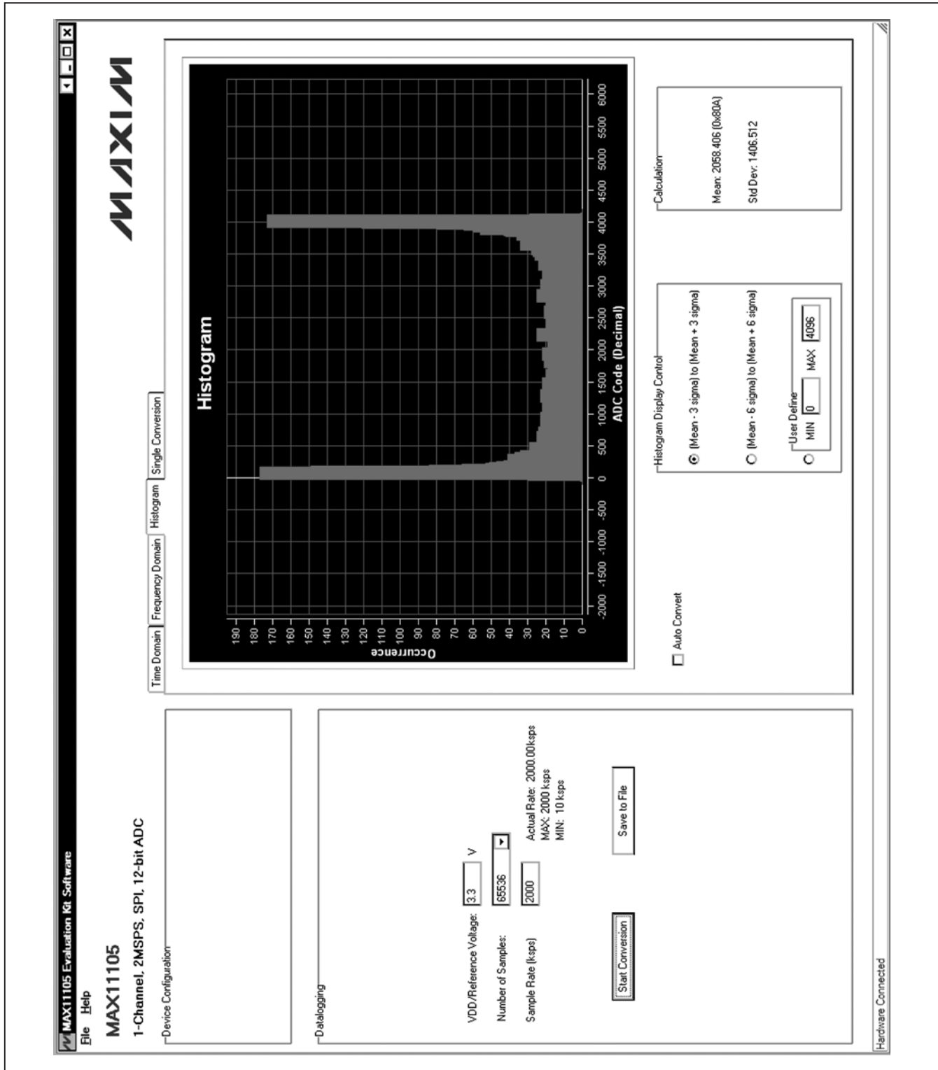
Figure 4. Histogram Tab
