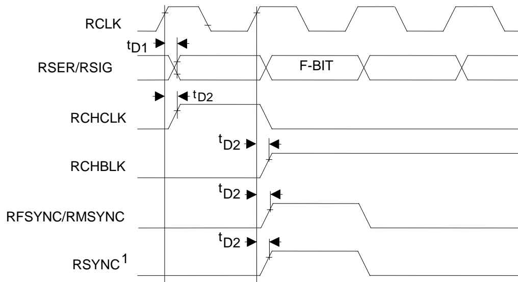
Figure 12-6. Receive Framing Timing—Backplane (T1 Mode)
