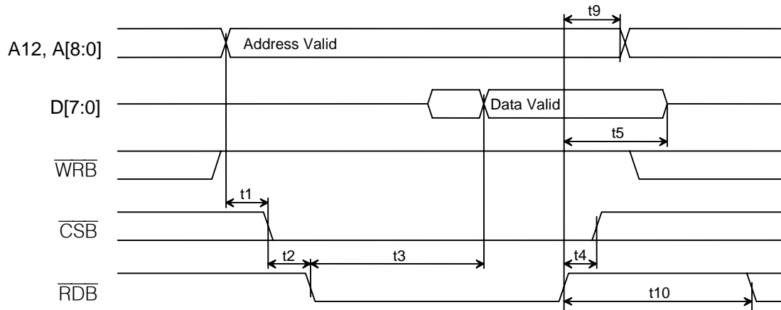
Figure 12-1. Intel Bus Read Timing (BTS = 0)
