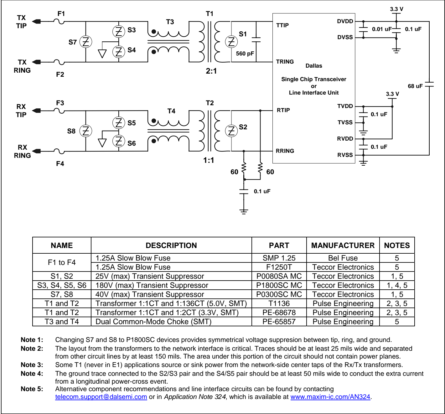
Figure 8-17. Basic Balanced Network Connections
