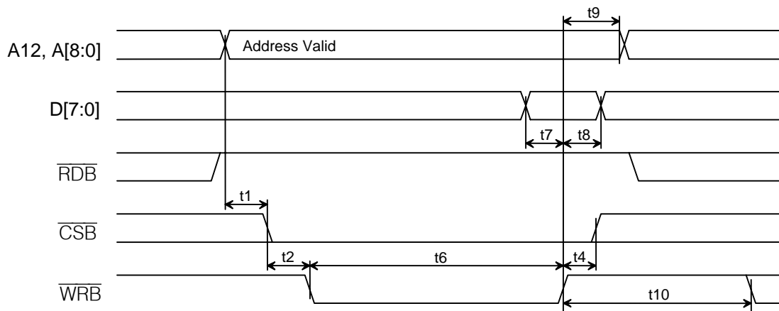
Figure 12-2. Intel Bus Write Timing (BTS = 0)
