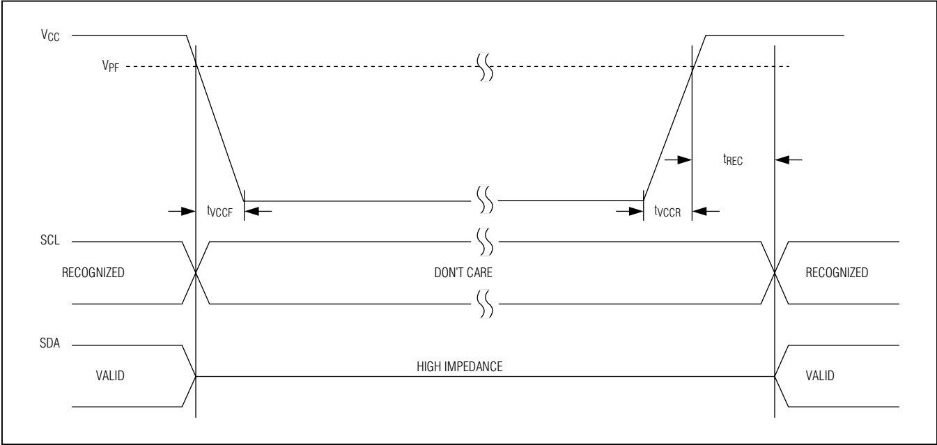
Figure 2. Power-Up/Power-Down Timing
