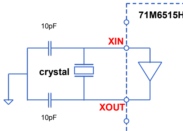
Figure 2-8: Oscillator Circuit
