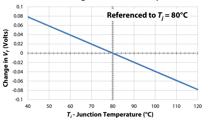
Forward Voltage vs Junction Temperature
