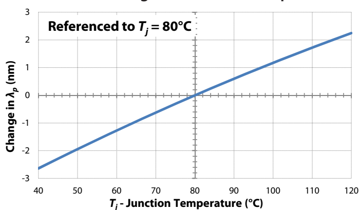
Peak Wavelength vs Junction Temperature
