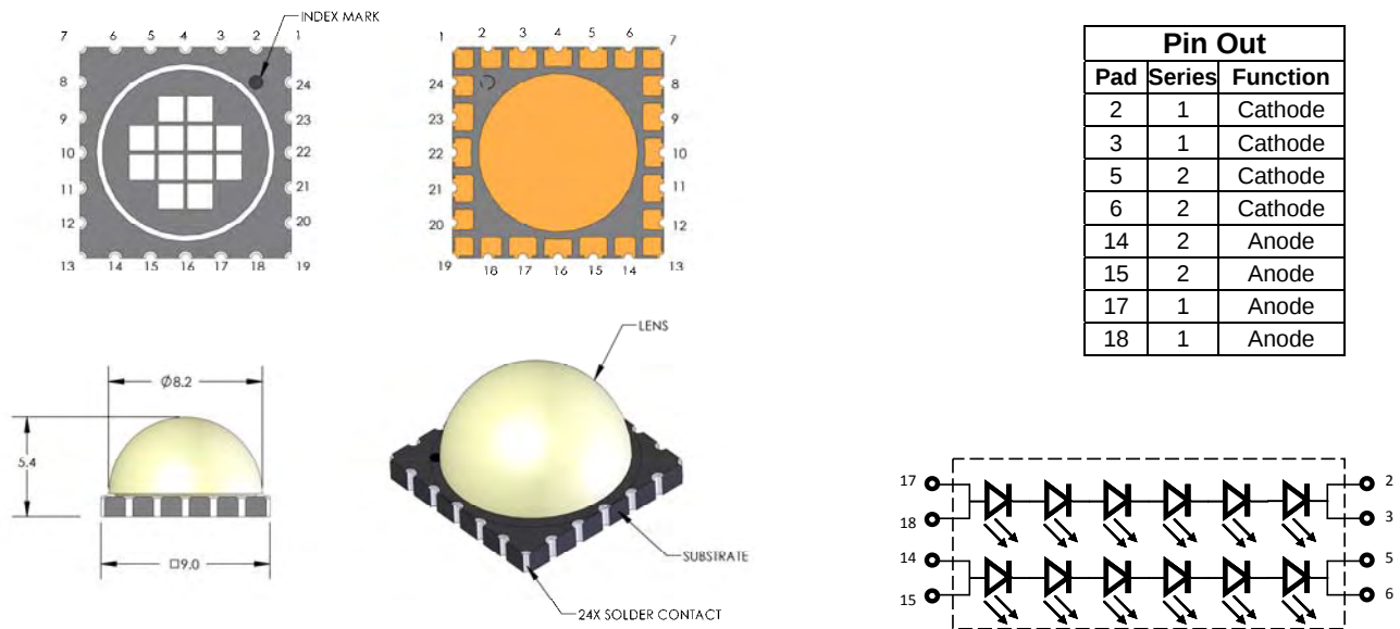
Figure 3: Package outline drawing.
