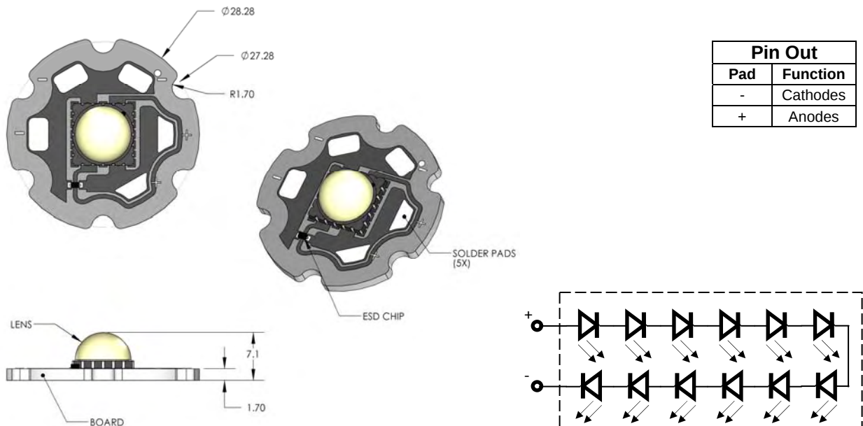
Figure 11: Standard MCPCB outline dimensions (mm).
