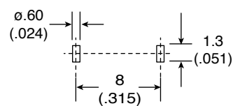
Mounting Hole
