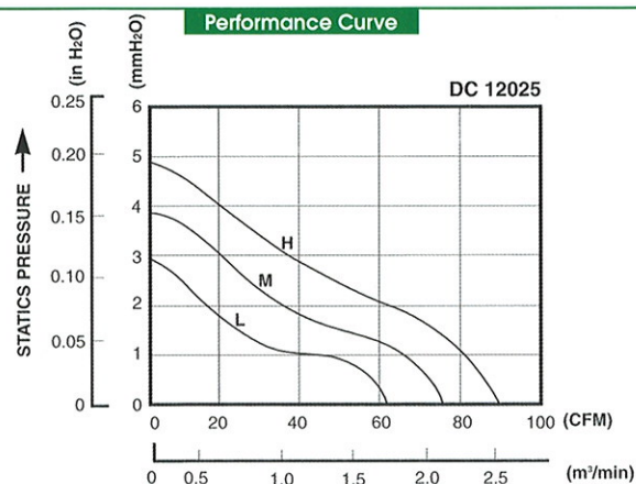
Performance Curve
