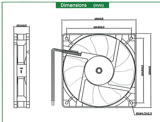
Dimensions (mm)
