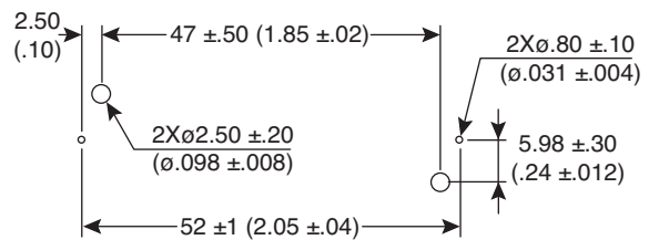
PCB/Mounting Layout
