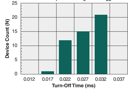
Typical Turn-Off Time (N=50, I_F=10mA , I_L=50mA_{DC} )
