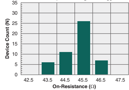
Typical On-Resistance Distribution (N=50, I_F=10mA , I_L=50mA_{DC} )
