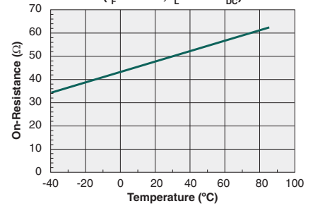
Typical On-Resistance vs. Temperature ( I_F=10\text{mA} , I_L=50\text{mA}_{DC} )
