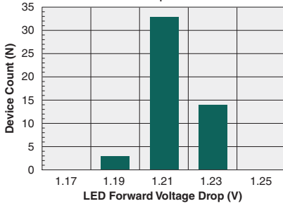
Typical LED Forward Voltage Drop (N=50, I_F=10mA )
