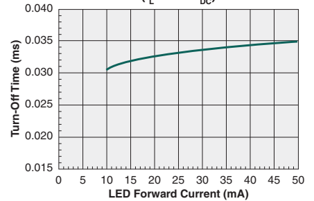
Typical Turn-Off Time vs. LED Forward Current ( I_L=50mA_{DC} )
