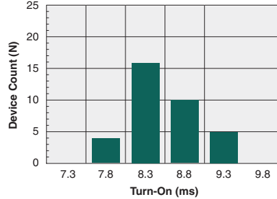
Typical Turn-On Time (N=35, I F =20mA, I L =1A DC )
