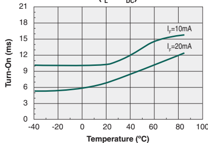
Typical Turn-On Time vs. Temperature (I L =1A DC )
