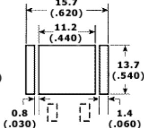
Recommended Heat Sink Solder Mask Opening
