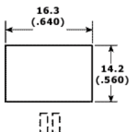
Recommended Cu Heat Spreader Drain Pad
