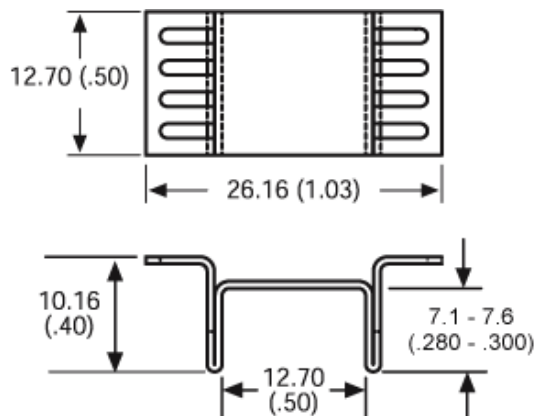
Recommended Cu Heat Spreader Drain Pad
