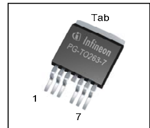
PG-T0263-7-3
