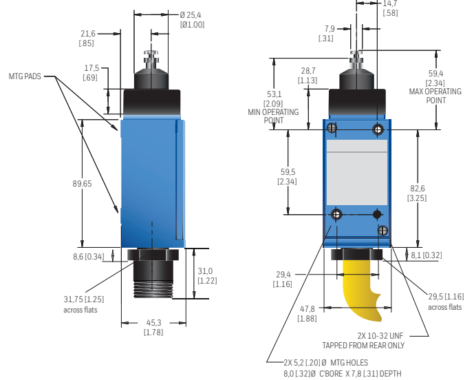
Figure 41. LSYV Top Adjustable Plunger (Momentary) DPDT (mm[in])
