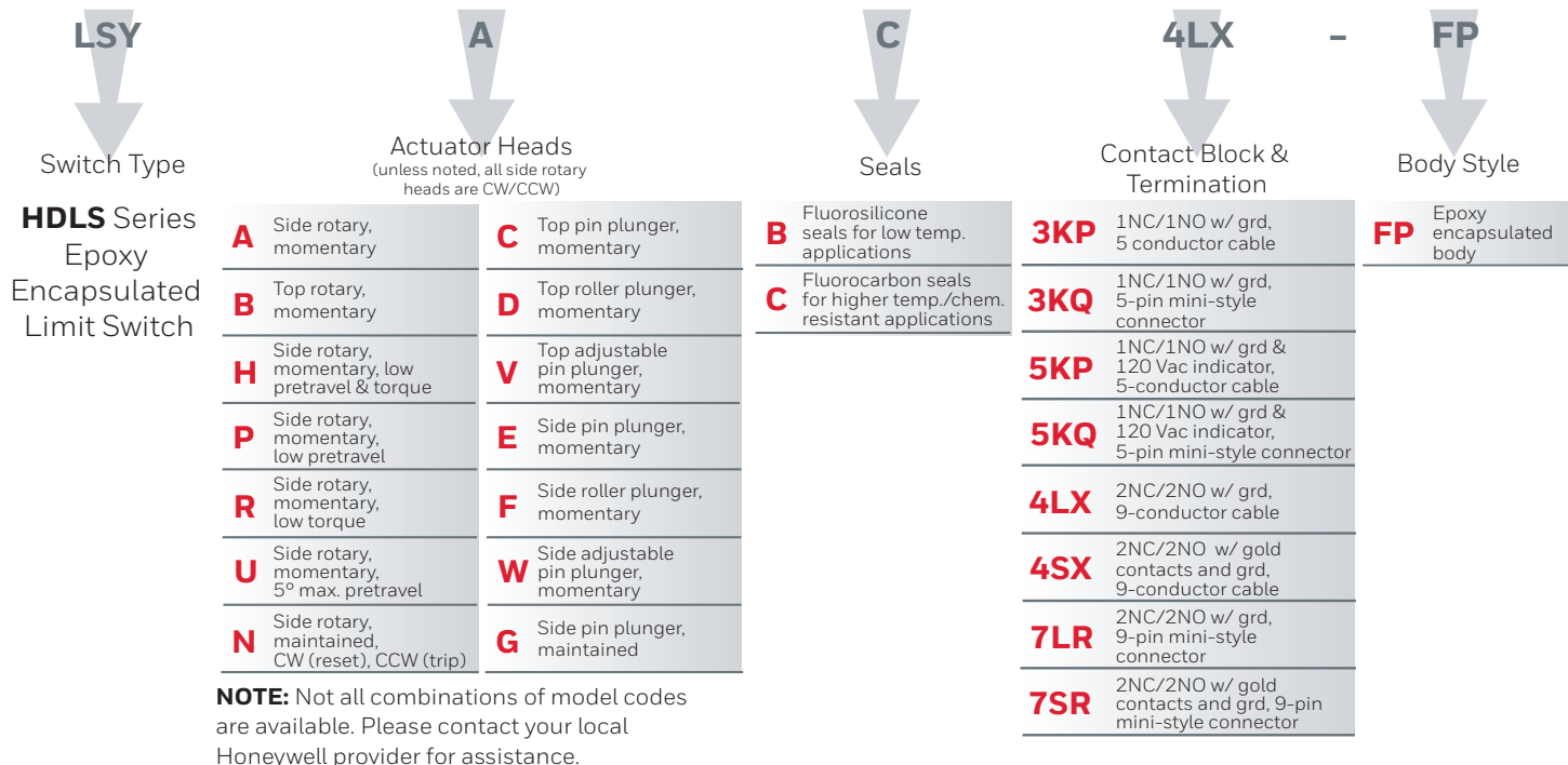
Figure 1. Product Nomenclature: Side Rotary and Plunger Versions
