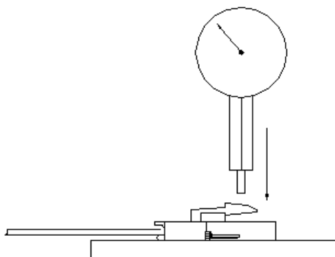
Figure 6 External Latch Testing
