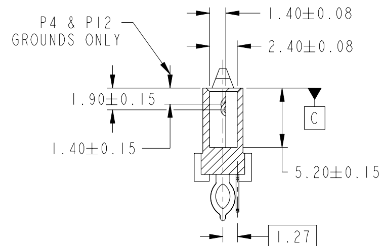
SECTION X-X
