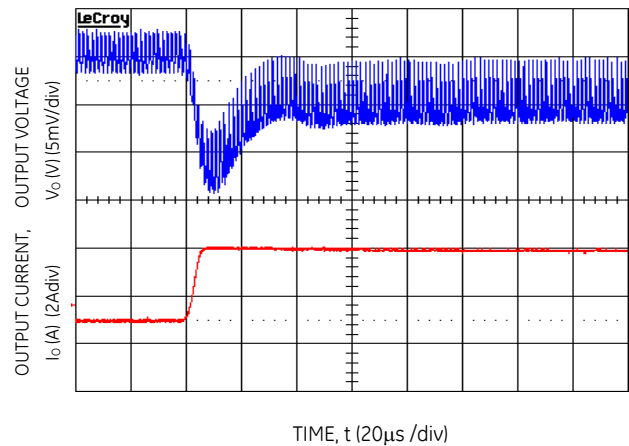
Figure 4. Transient Response to Dynamic Load Change from 50% to 100% at 9Vin, C_{out}=2\times 47\mu\text{F}+4\times 330\mu\text{F} , C_{Tune}=33\text{nF} , R_{Tune}=178
