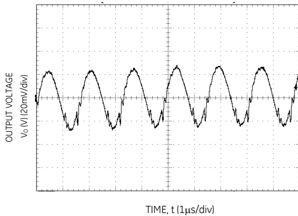
Figure 27. Typical output ripple and noise ( C_o=10\mu\text{F} ceramic, V_{IN} = 12\text{V} , I_o = I_{o,max} ).
