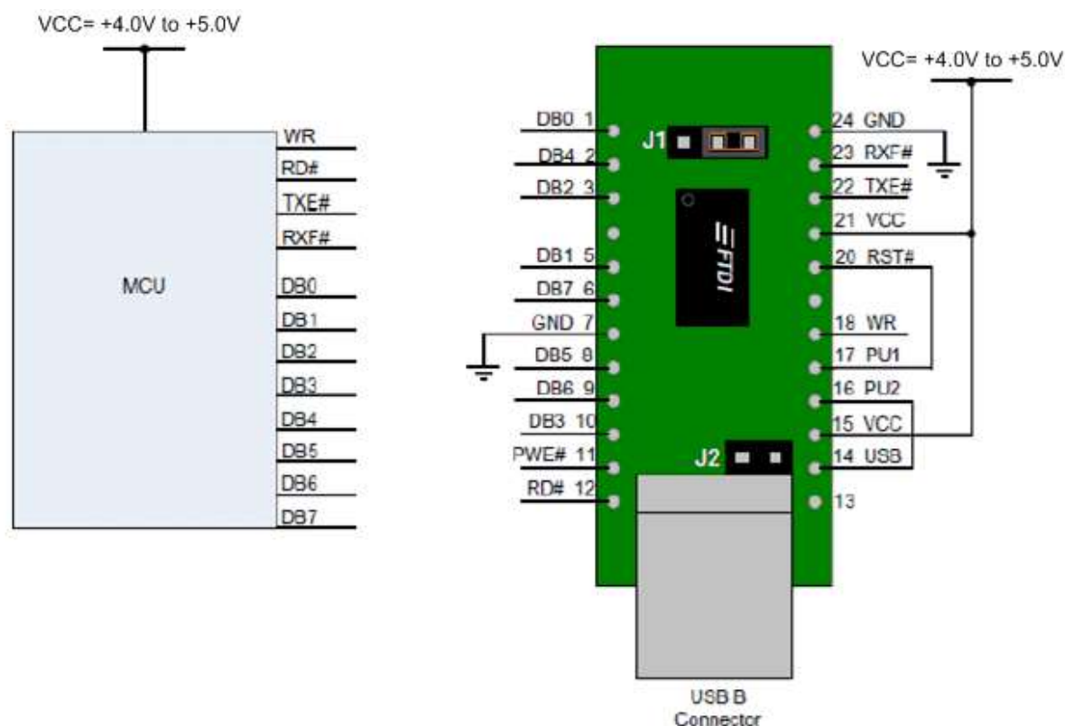
Figure 7.2 Self-Powered Configuration
